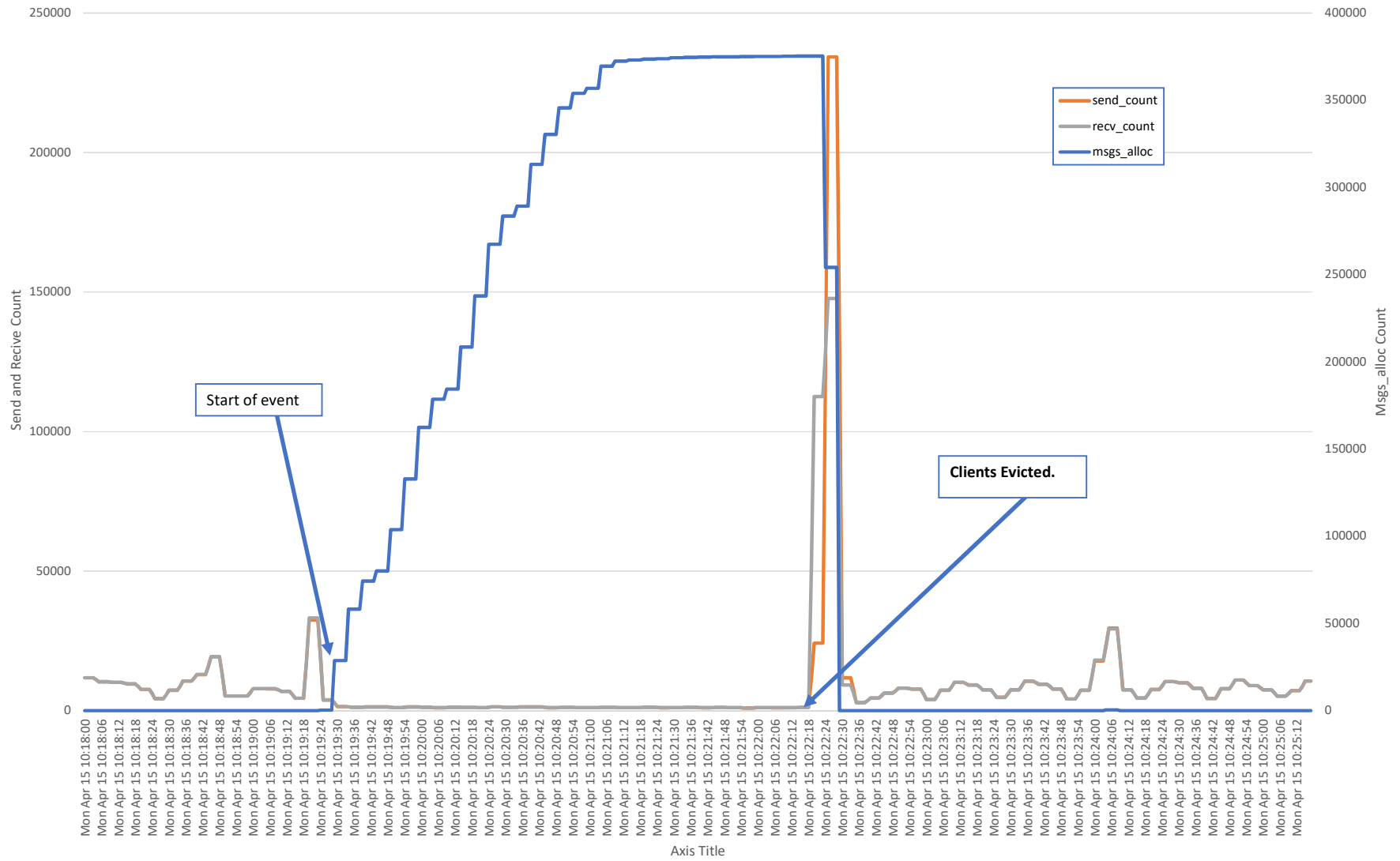
Lnet Metrics During Client Eviction
